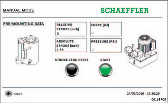
Figure 23 MANUAL MODE Screen 1
