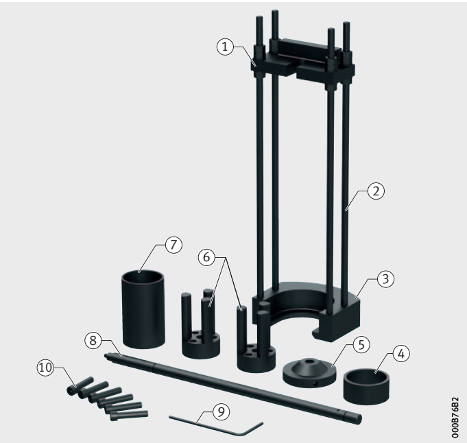
Figure 4 Tool set TOOL-RAILWAY-AXLE
