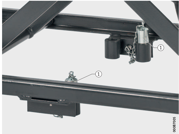
① Pins for securing against unintentional lowering
