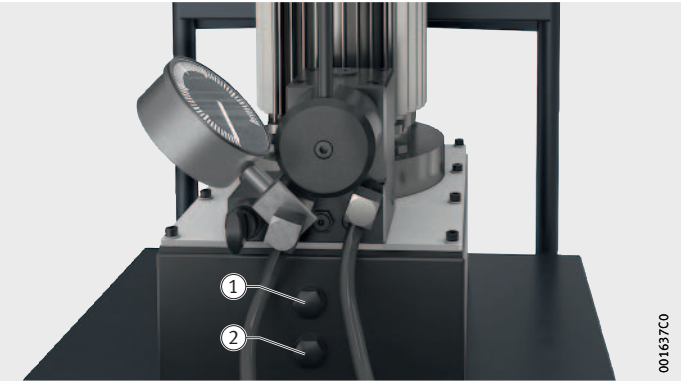
Figure 54 Checking the hydraulic oil level
